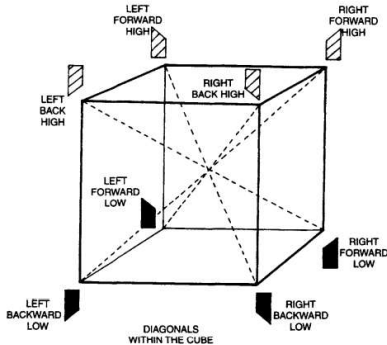
Figure 62. Diagonals within the cube.
